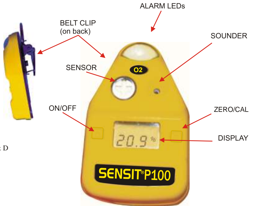
SENSIT P100 comes with belt clip and instruction manual
